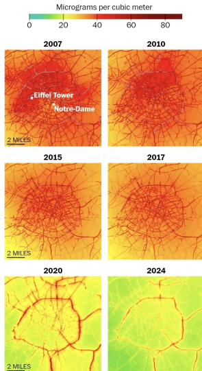
Average nitrogen dioxide concentration in Paris
